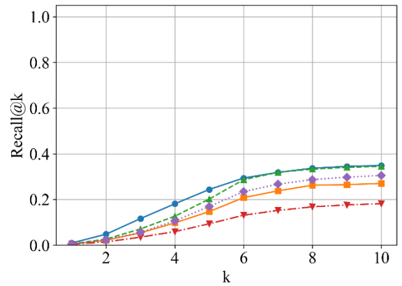
(f) R@k on WWk large
